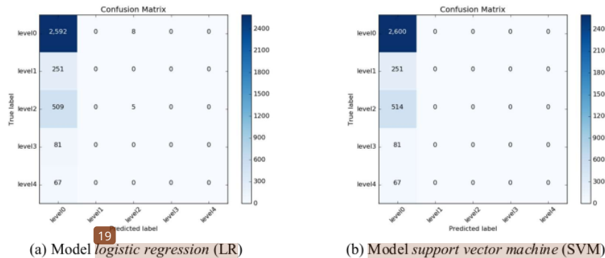
Gambar 3 Confusion Matrix
